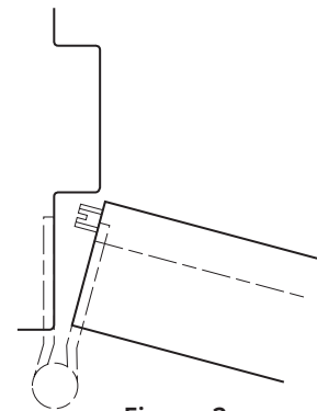
Figure 2 Semi-Mortise Mounted
