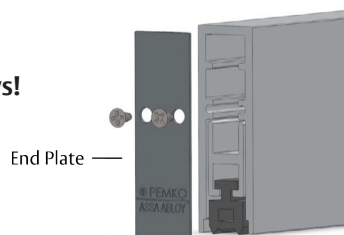
Figure 4 - Properly Installed End Plate
