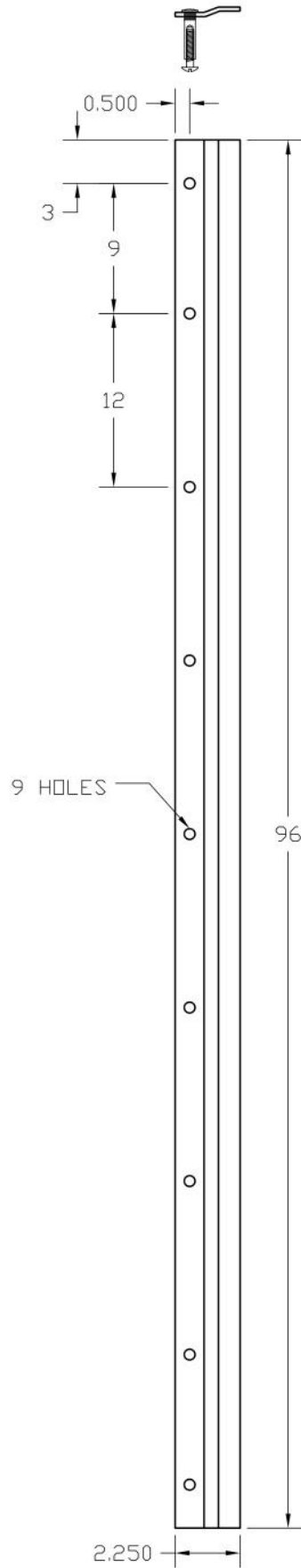
3572 - 96" LENGTH
