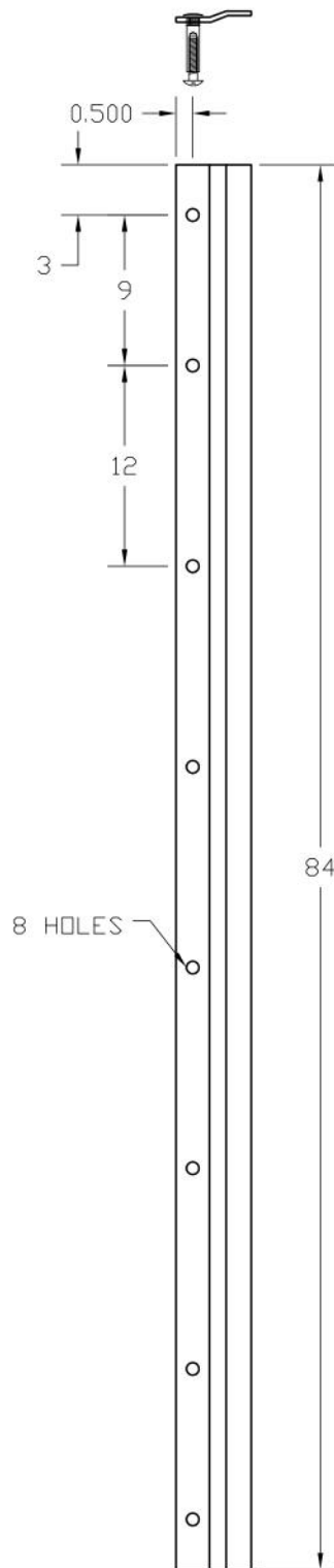
3572 - 84" LENGTH
