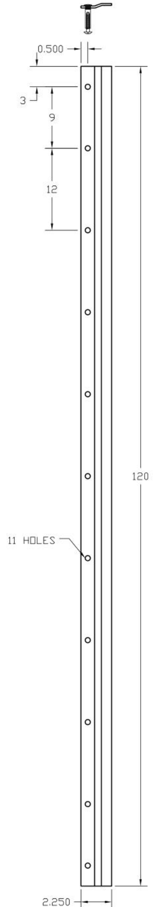
3572 - 120" LENGTH
