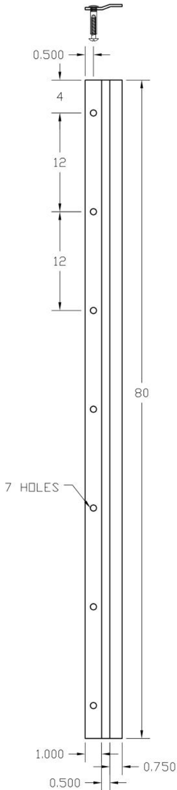
3572 - 80" LENGTH
