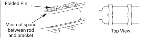
DETAIL 2 - COTTER PINS
