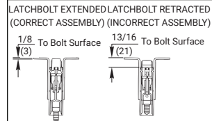
DETAIL 3 - TOP LATCH
