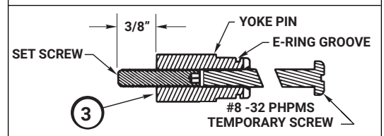
DETAIL 1 - YOKE PIN ASSEMBLY
